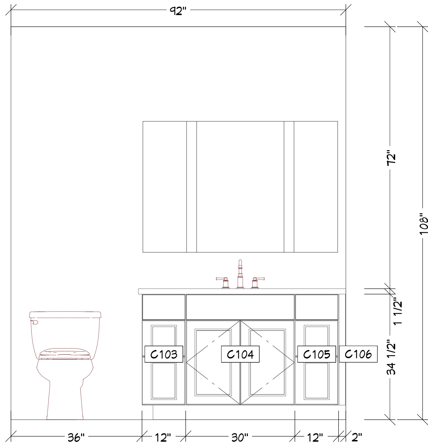
Q 15 In-Law Bath 3/4 in = 1 ft
