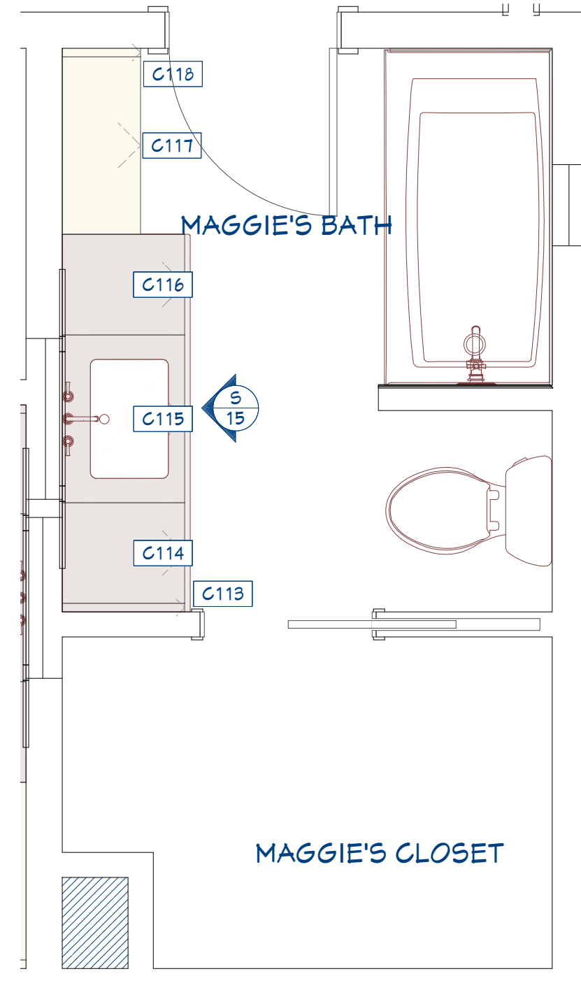
15 NKBA - Kitchen & Bath Plan 1/2" 1/2 in = 1 ft
