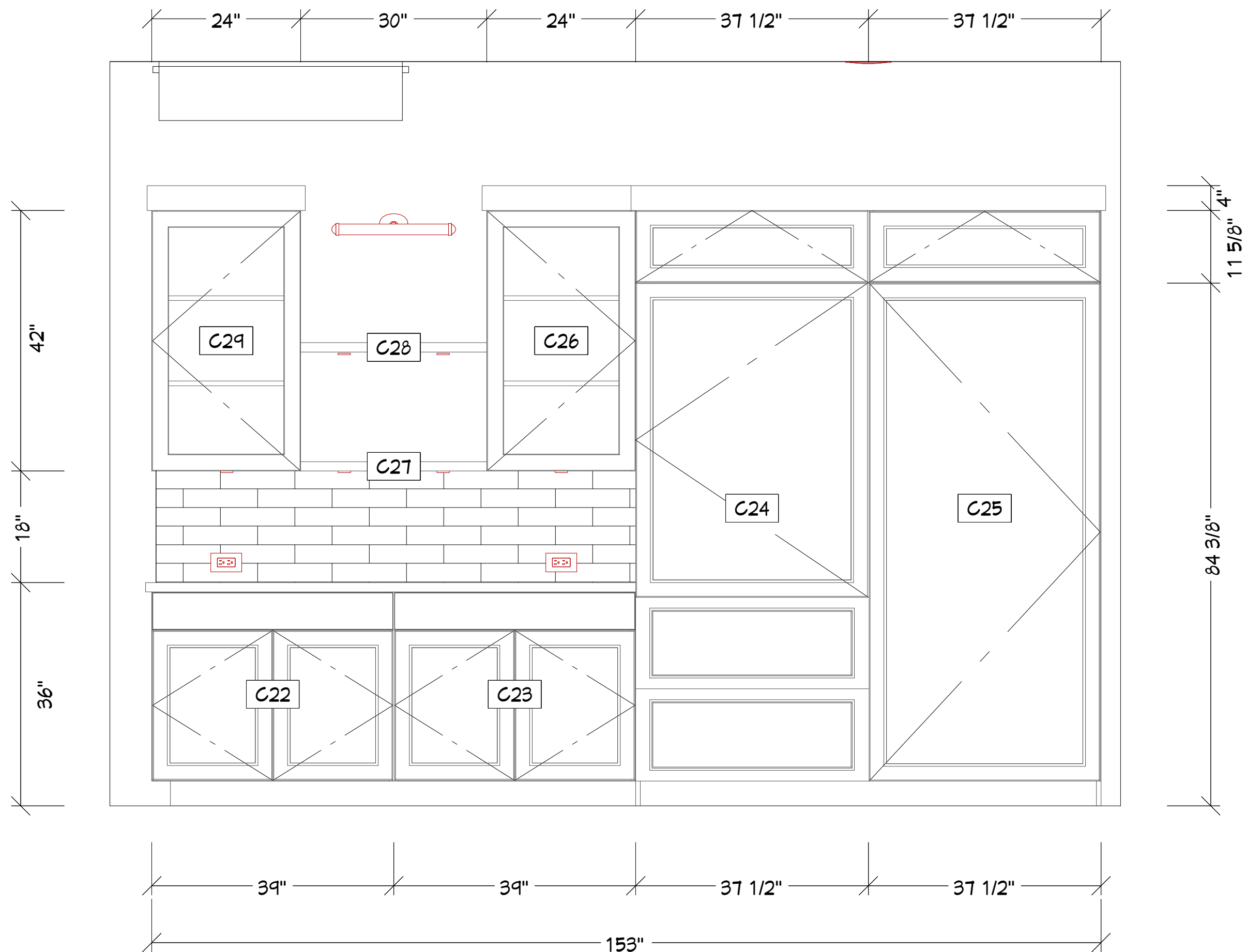
C 8 Refrigerator Wall Side 3/4 in = 1 ft
