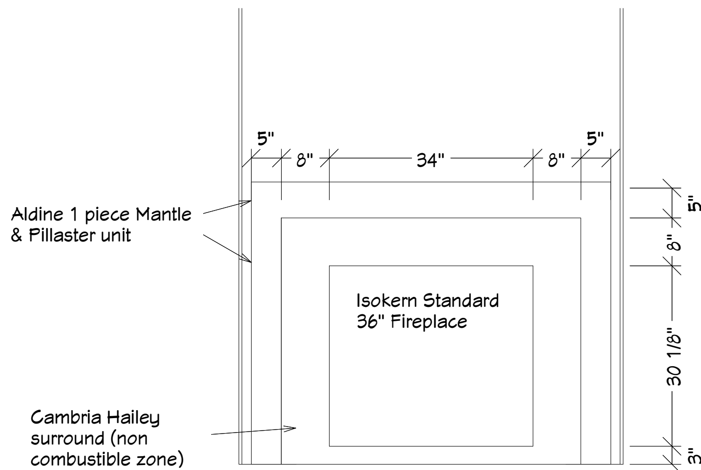
PFP 18 Primary fireplace 3/4 in = 1 ft
