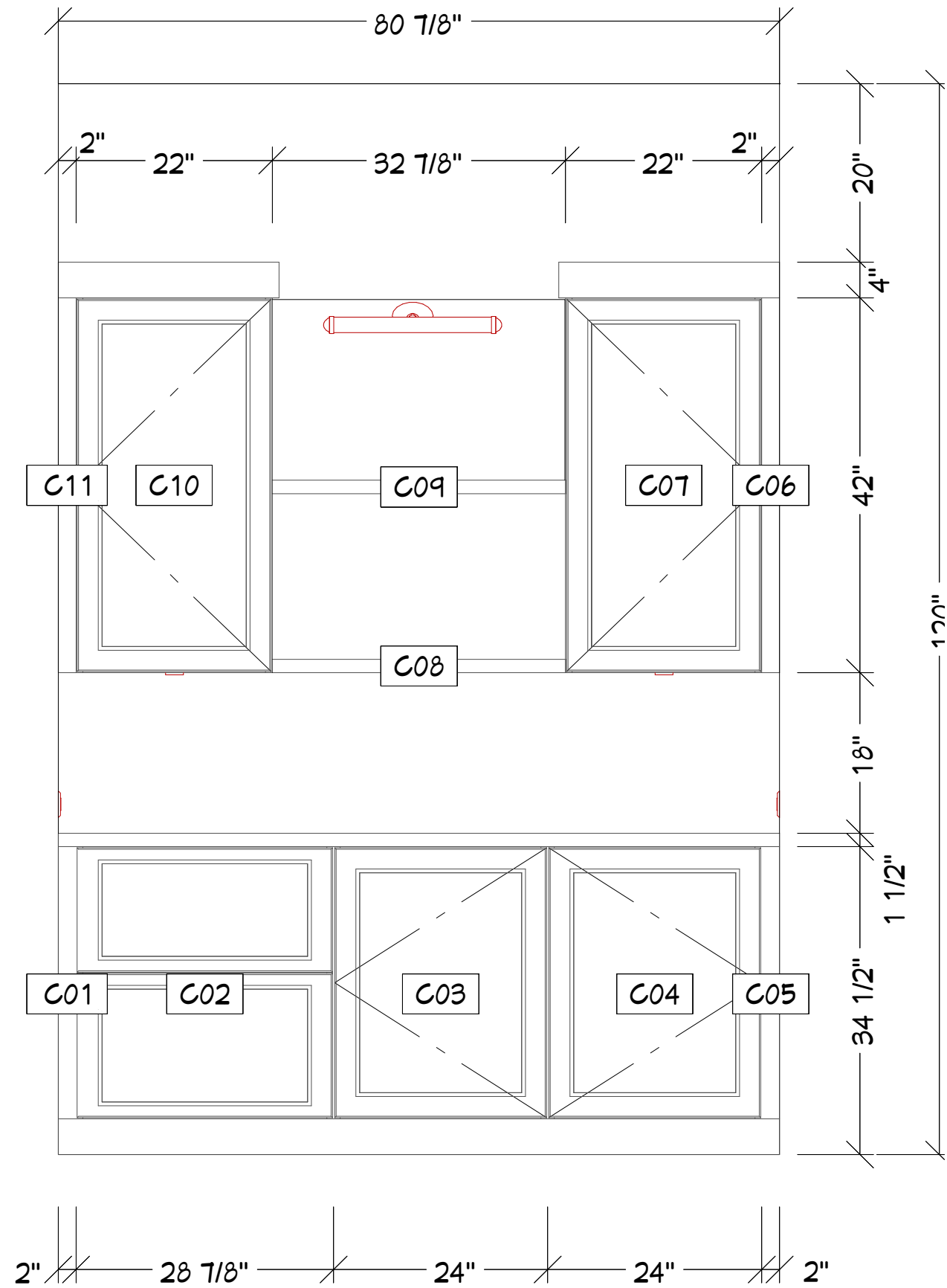
A 7 Bar- Wine/Bev Fridge Side 3/4 in = 1 ft
