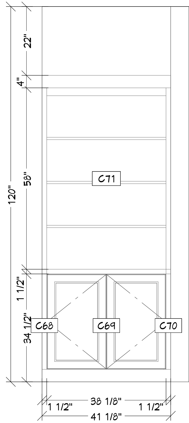
K 11 Hallway Built-In 3/4 in = 1 ft
