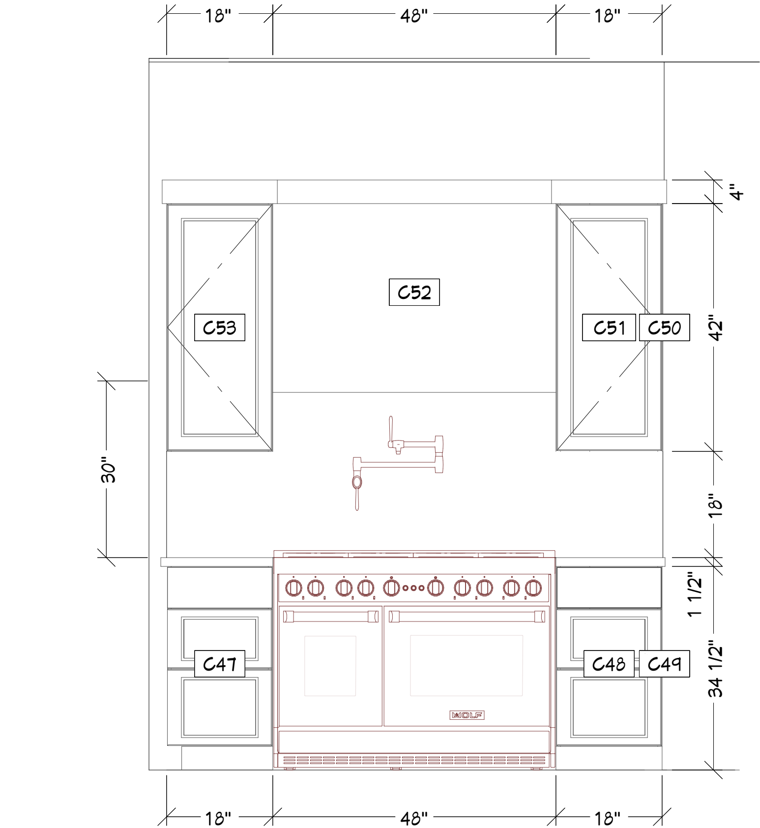
E 9 Range Wall 3/4 in = 1 ft
