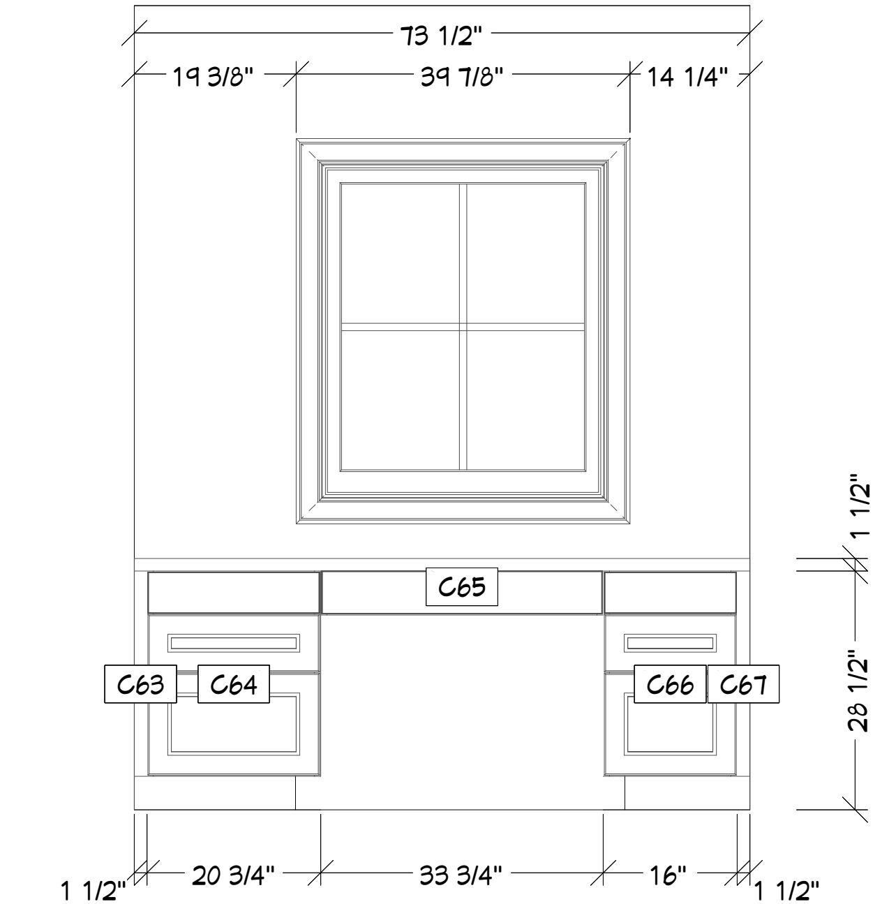
J 9 Servery Window Side 3/4 in = 1 ft
