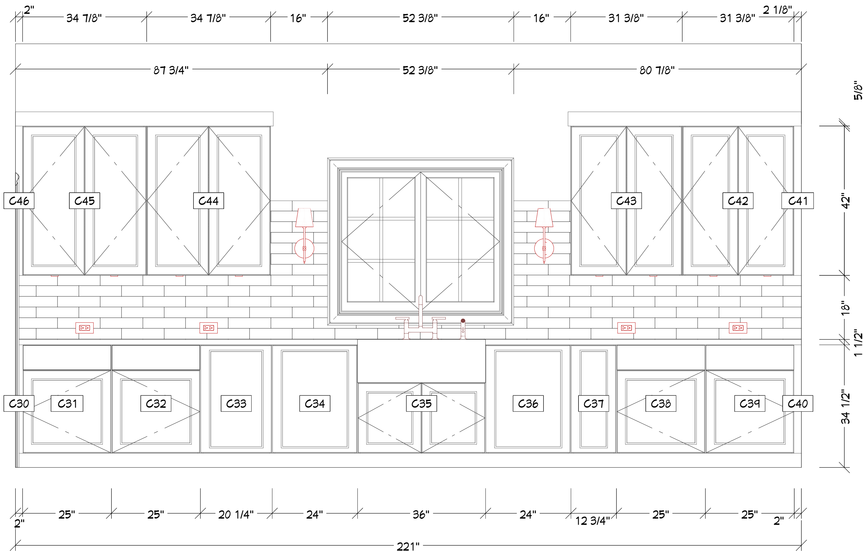
D 8 Kitchen Sink Wall 3/4 in = 1 ft
