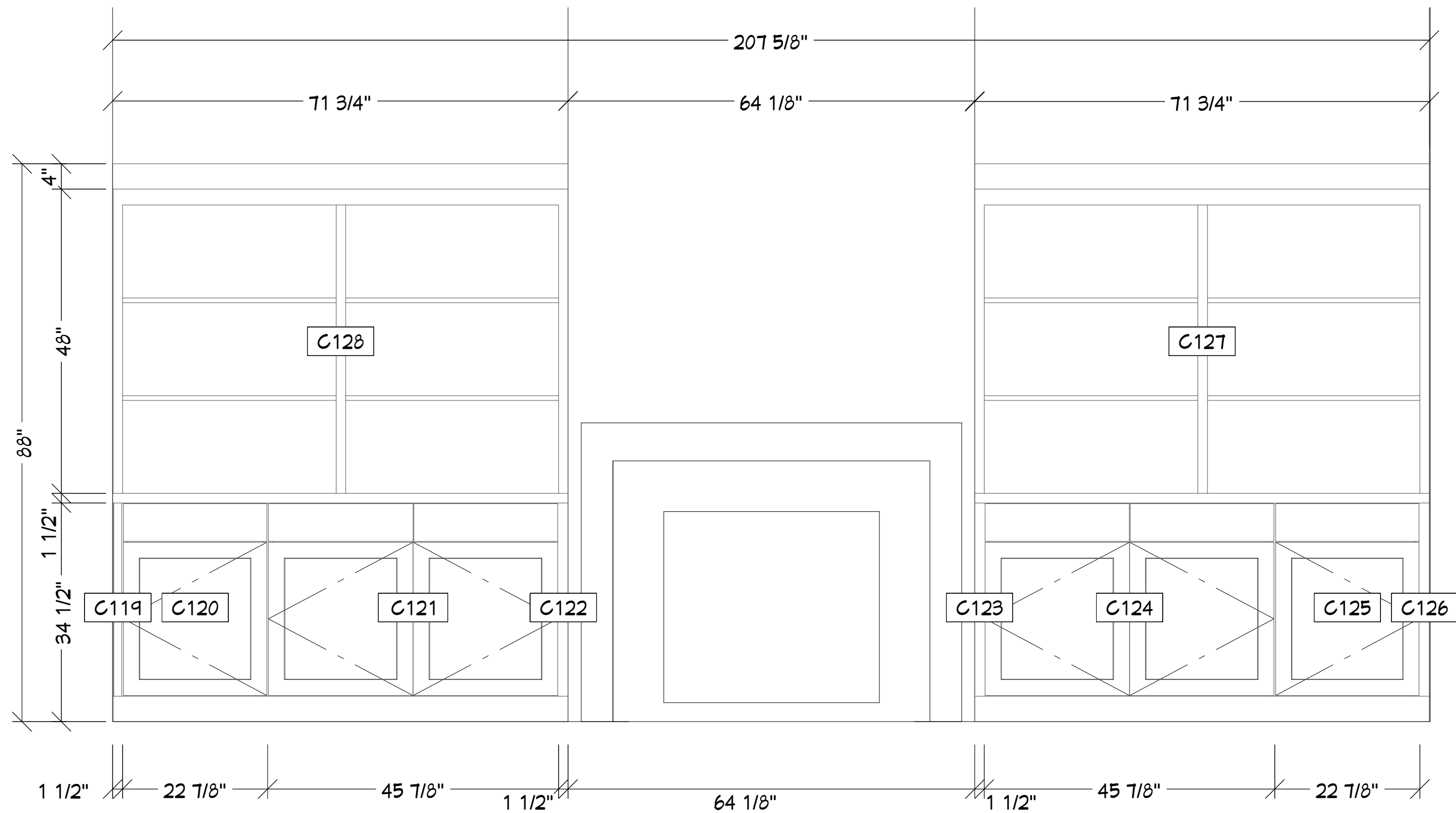
T 18 Primary Builtin 3/4 in = 1 ft
