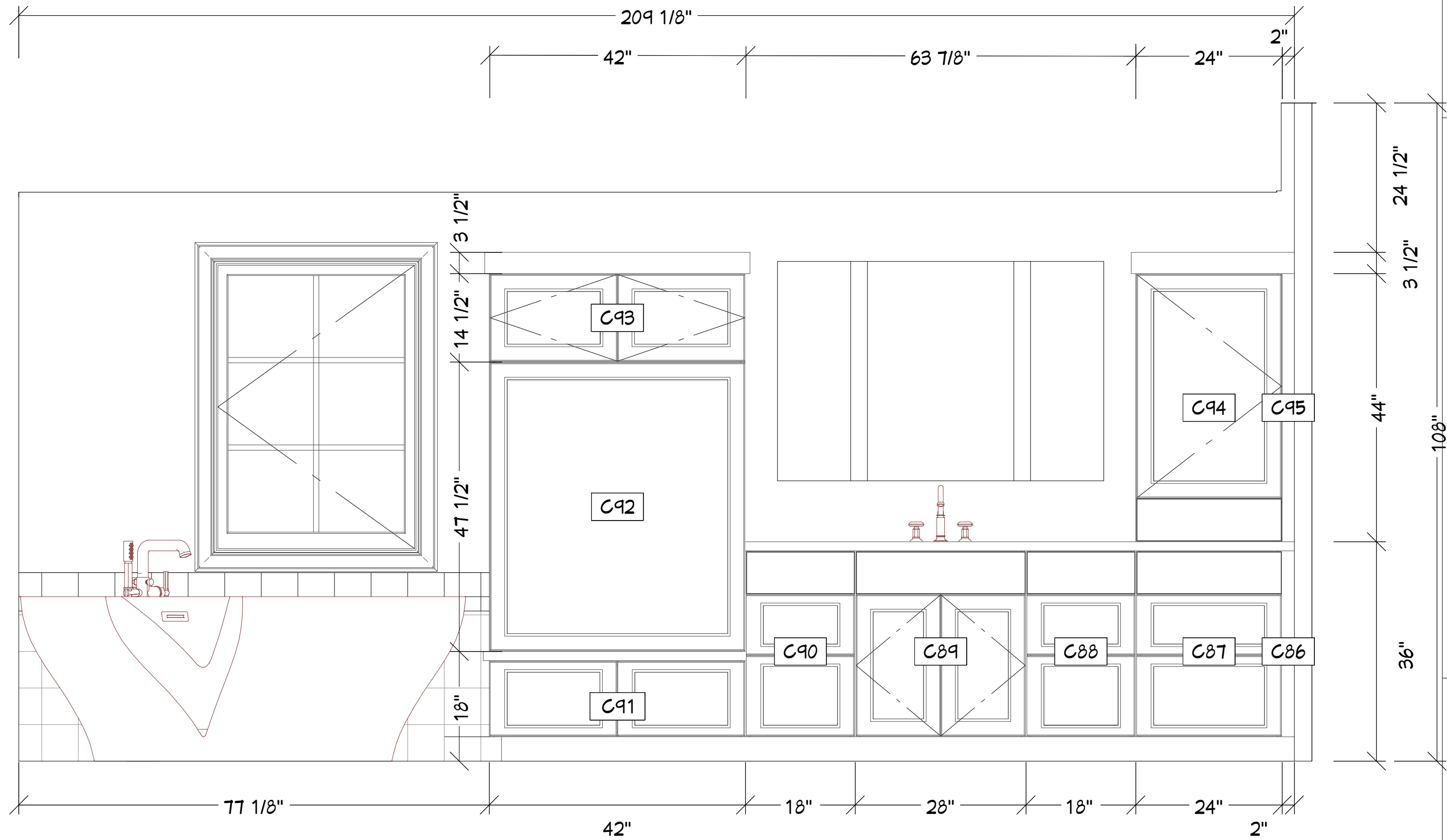
O 13 Primary Bath R 3/4 in = 1 ft
