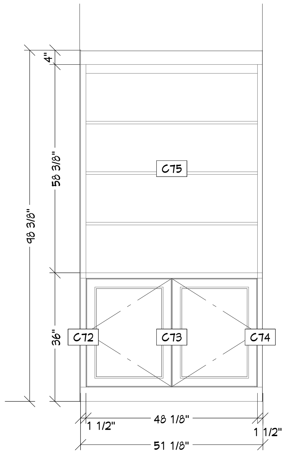
L 11 Living Room Built-In 3/4 in = 1 ft
