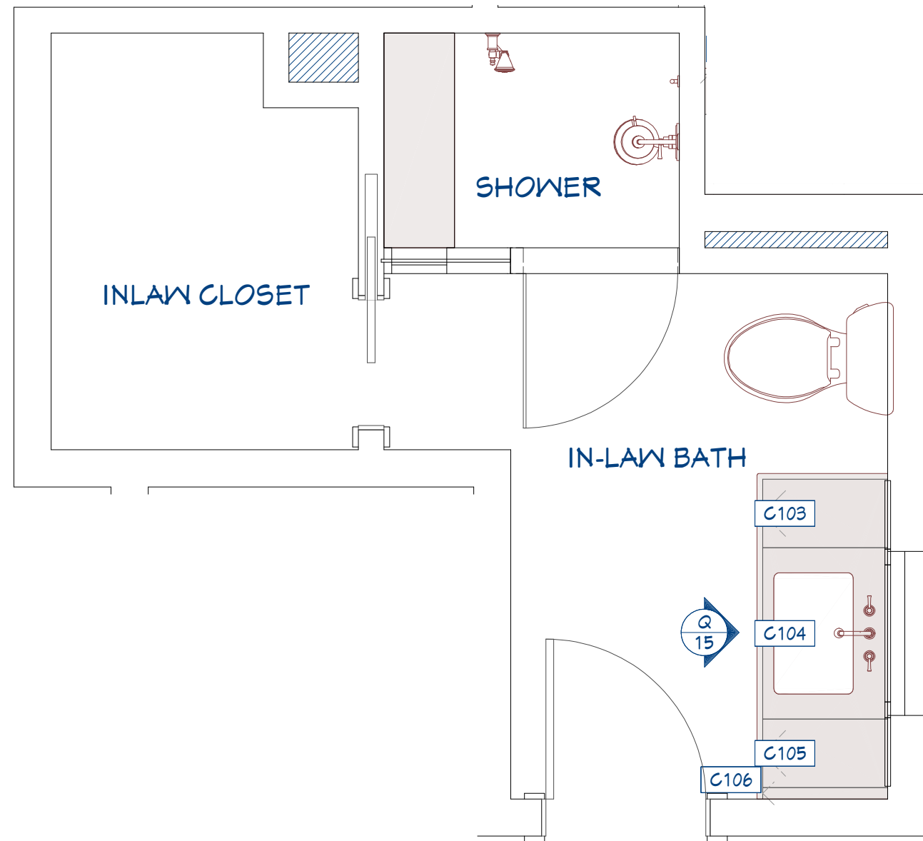
15 NKBA - Kitchen & Bath Plan 1/2" 1/2 in = 1 ft
