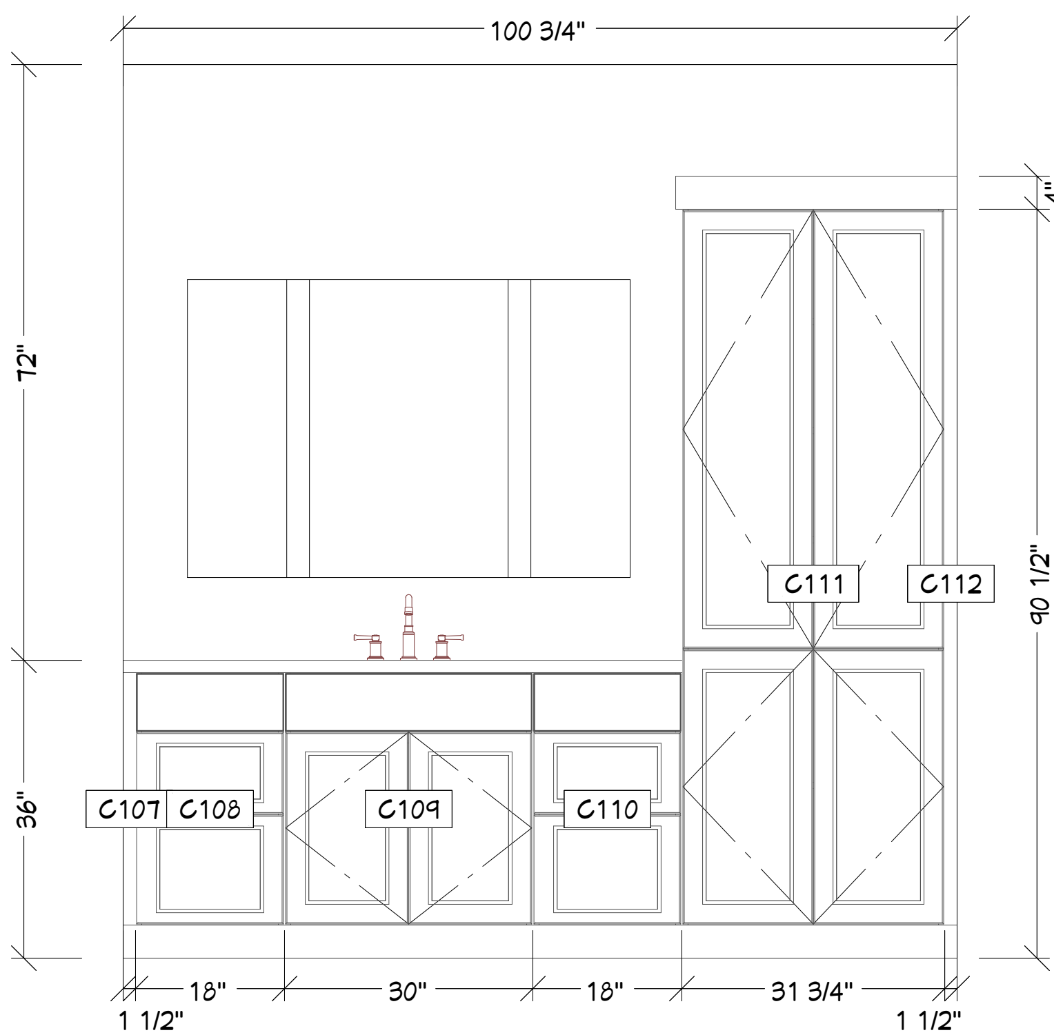
R 15 Flex Bath 3/4 in = 1 ft
