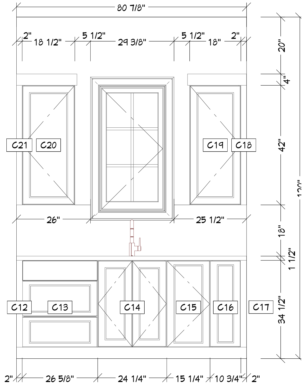
B 7 Bar Window Side 3/4 in = 1 ft
