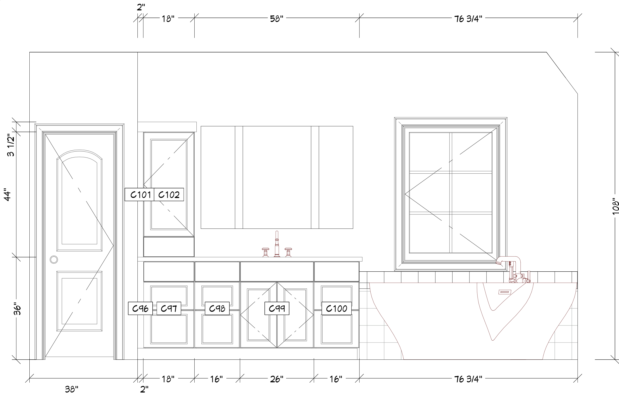
O 13 Primary Bath R 3/4 in = 1 ft
