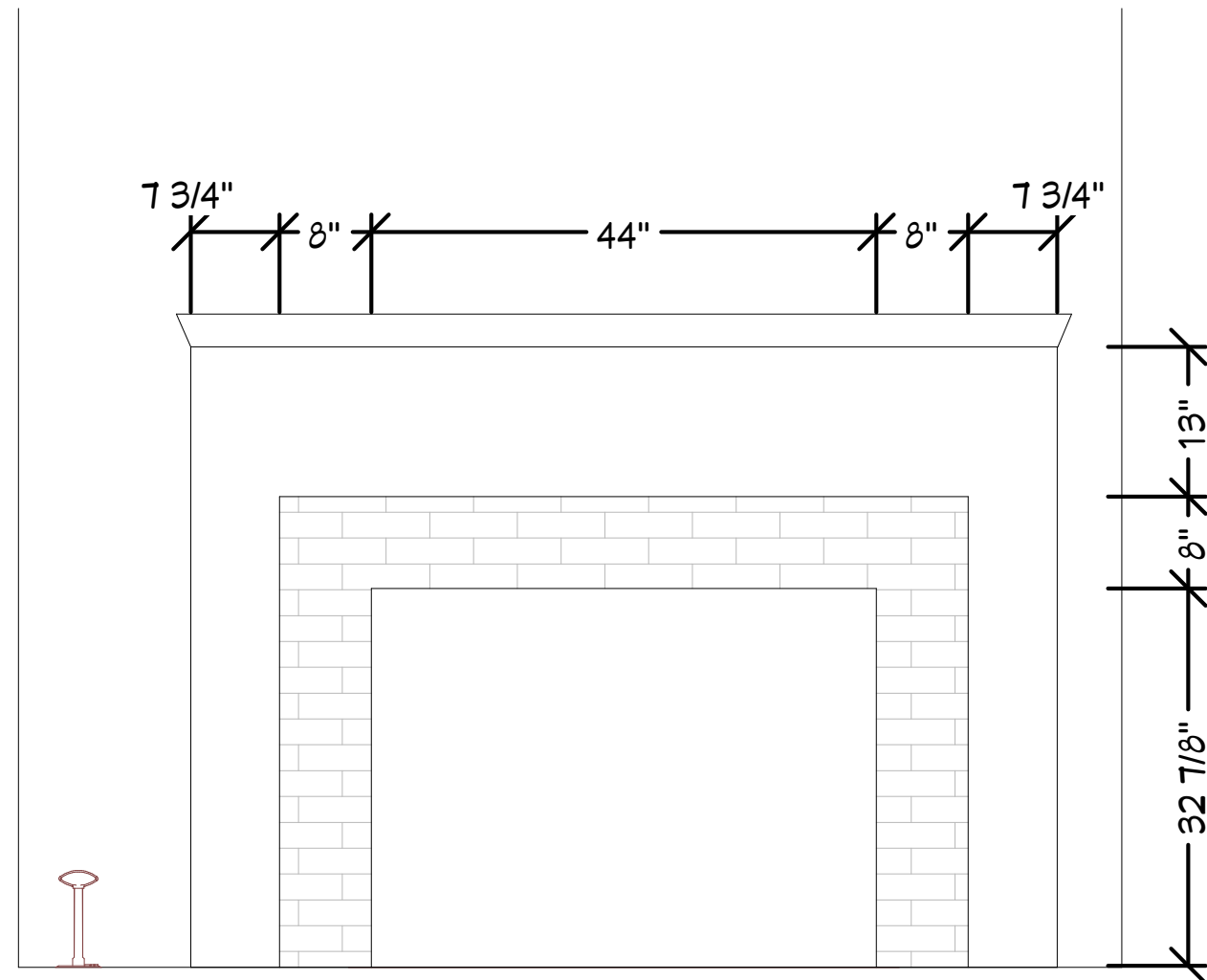
LFP 11 Living room FP 3/4 in = 1 ft
