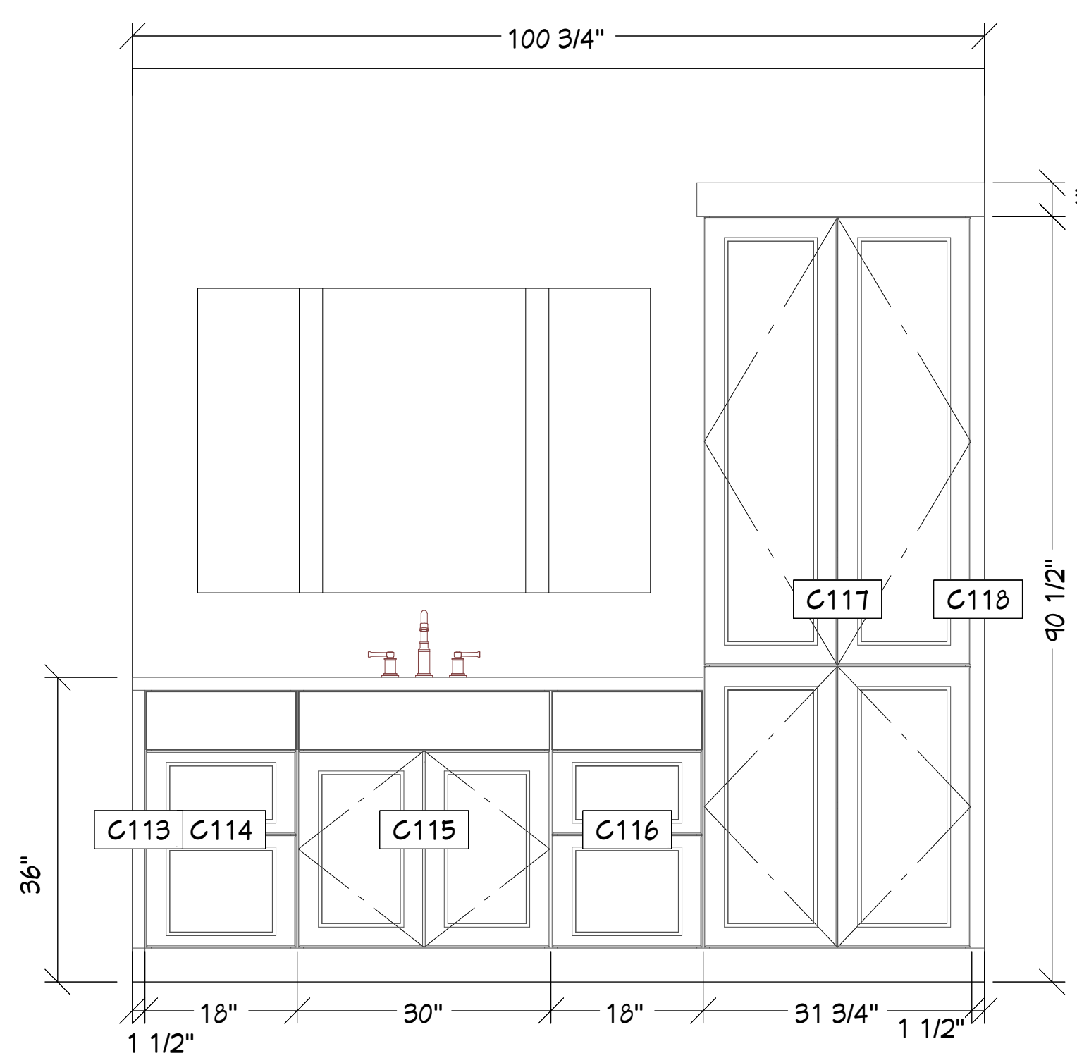
S 15 Maggie's Bath 3/4 in = 1 ft
