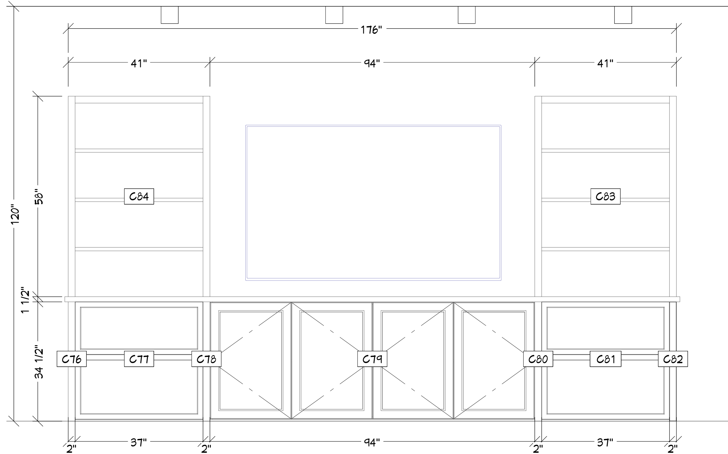
M 11 Living Room Media Center 3/4 in = 1 ft
